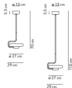
TRATTO STANDARD LENGTHS 2 TIGES INCLUDED
