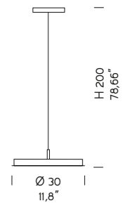
0615 LED 9W
